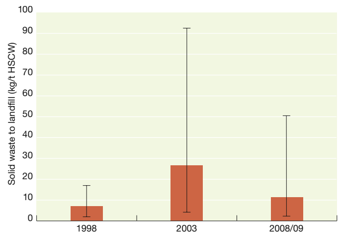
Figure 13: Comparison of solid waste sent to landfill for 1998, 2003 and 2008–09
