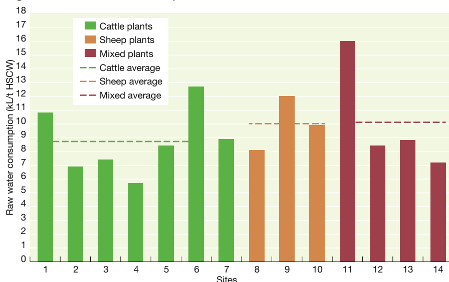
Figure 1: Raw water consumption
