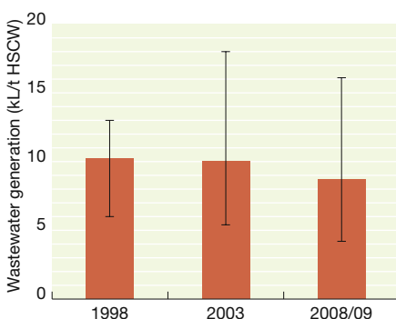
Figure 5: Comparison of wastewater generation for 1998, 2003 and 2009
