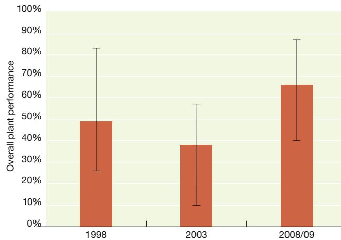
Figure 15: Comparison of overall plant performance for 1998, 2003 and 2009
